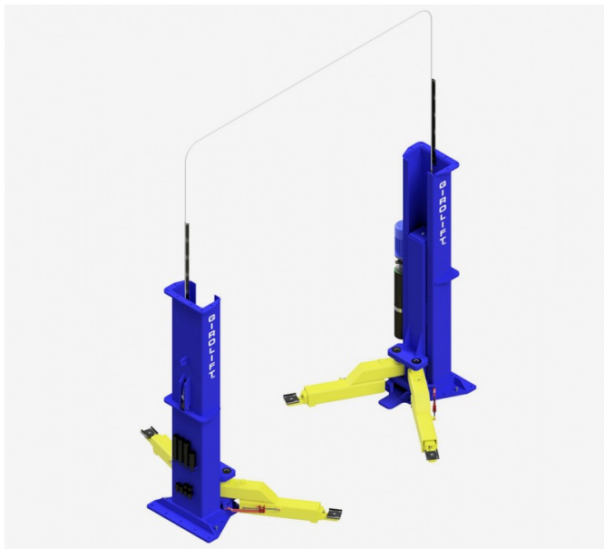
Pneumatic swing arm
