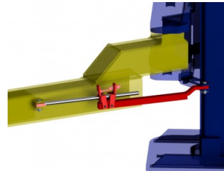
Swing arm restraint
