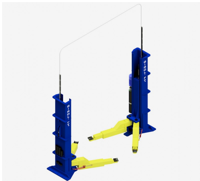
Pneumatic swing arm
