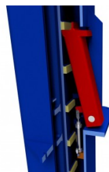
Automatic load holding system
